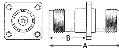
Figure 2 (Panel mount)
