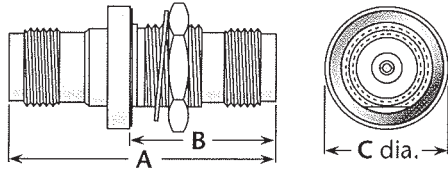
Figure 1 (Bulkhead mount)
